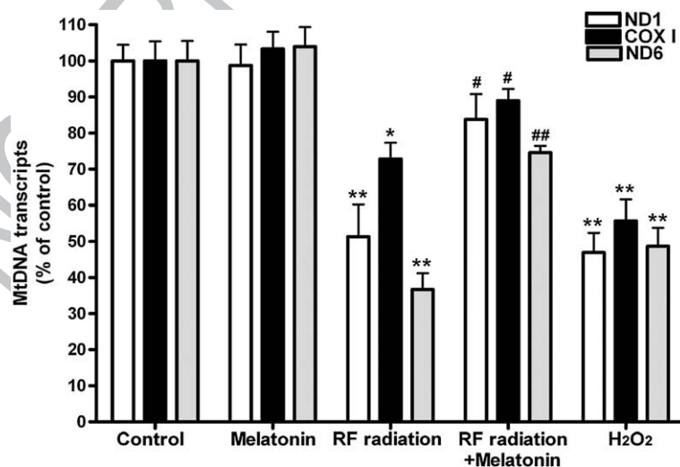
Fig. 4 – Decrease of mtRNA transcripts levels after RF radiation. Quantitative real-time PCR was used to measure the levels of mtRNA transcripts. The amounts of mtRNA were normalized to the internal control, \beta -actin. ** p < 0.01 , * p < 0.05 versus sham-exposed control group and melatonin group, ## p < 0.01 , # p < 0.05 versus RF radiation group. Values are means \pm SE, n = 6 .
