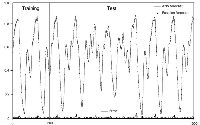
FIG. 3: COMPARATIVE BETWEEN THE RANN FORECAST AND THE FUNCTION FORECAST (4)
