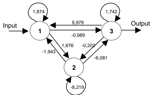
FIG. 2: RANN THAT EMULATE THE MACKEY-GLASS FUNCTION
