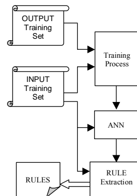
FIG. 1: RULE EXTRACTION PROCESS
